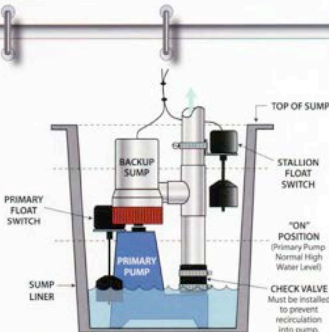
STANDARD INSTALLATION
